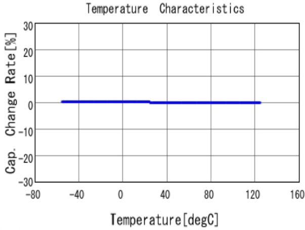
■ GRM1555C1H220JA01 C-Temp. capchange, DCOV, AC1Vrms
