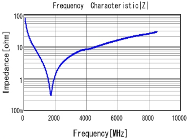
■ GRM1555C1H220JA01 |Z| DC0V, 25degC
