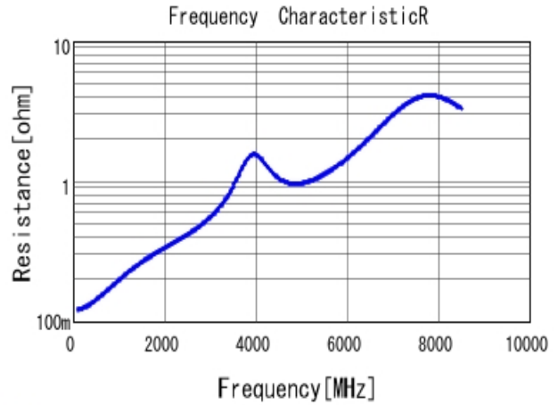
■ GRM1555C1H220JA01 R DC0V, 25degC
