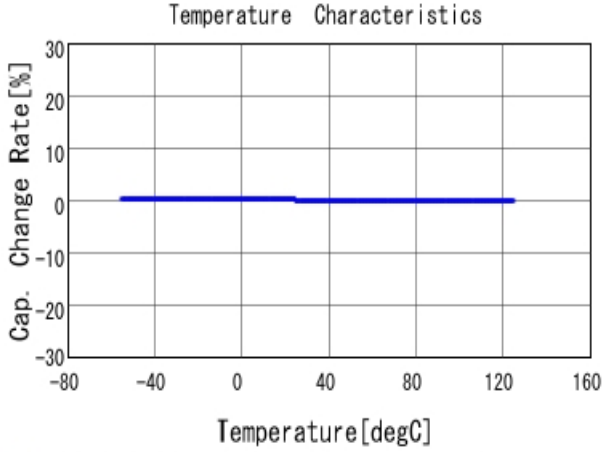
■ GRM1555C1H200JA01 C-Temp. capchange, DCOV, AC1Vrms
