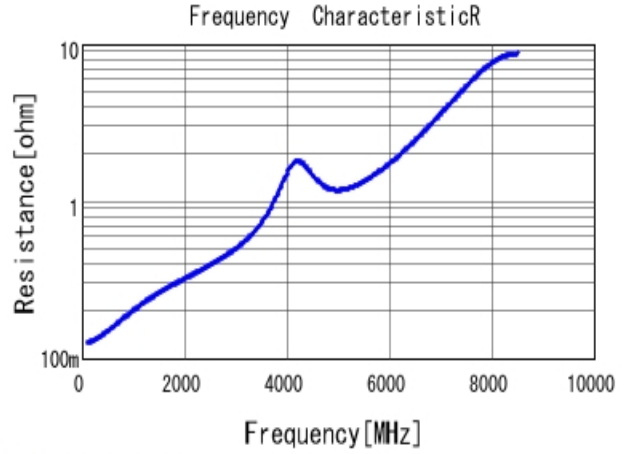
■ GRM1555C1H200JA01 R DC0V, 25degC
