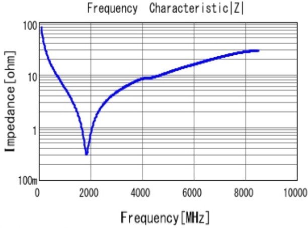
■ GRM1555C1H200JA01 |Z| DC0V, 25degC
