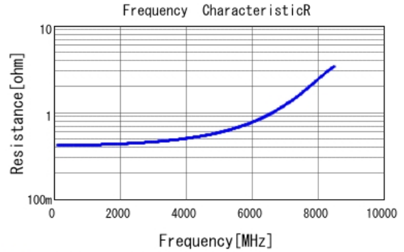
■ GRM1555C1H1R8CA01 R DCOV, 25degC
