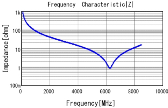
■ GRM1555C1H1R8CA01 |Z| DCOV, 25degC
