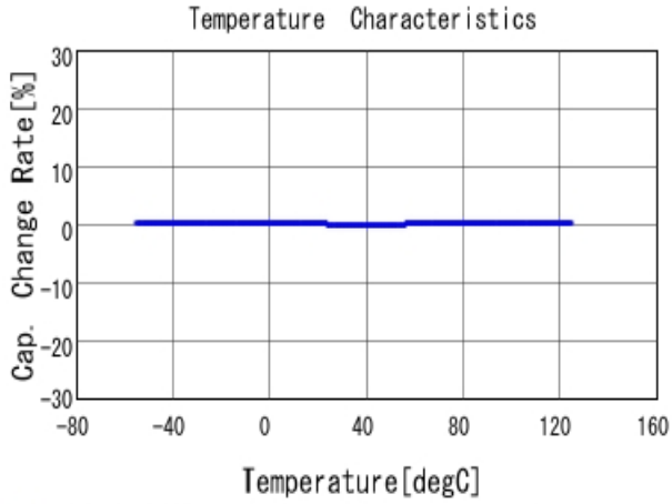
■ GRM1555C1H1R5WA01 C-Temp. capchange, DCOV, AC1Vrms
