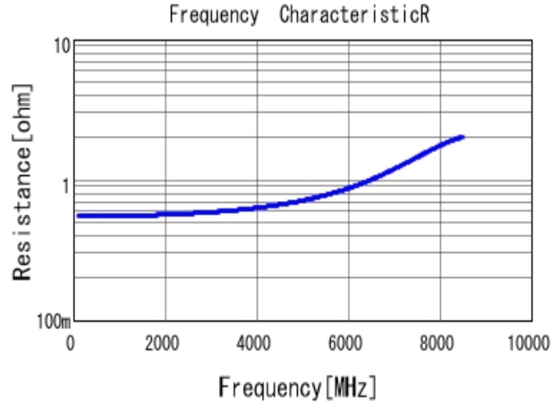
■ GRM1555C1H1R5WA01 R DCOV, 25degC
