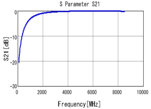
■ GRM1555C1H1R5WA01 S21 DCOV, 25degC
