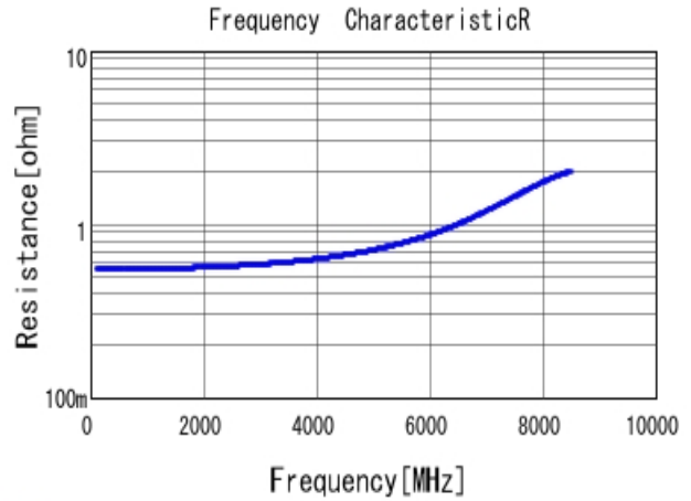
■ GRM1555C1H1R5CA01 R DCOV, 25degC
