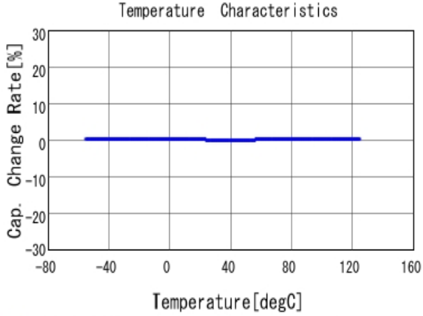
■ GRM1555C1H1R5CA01 C-Temp. capchange, DCOV, AC1Vrms
