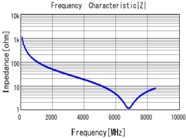
■ GRM1555C1H1R5CA01 |Z| DCOV, 25degC
