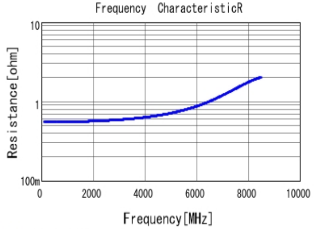
■ GRM1555C1H1R5BA01 R DCOV, 25degC
