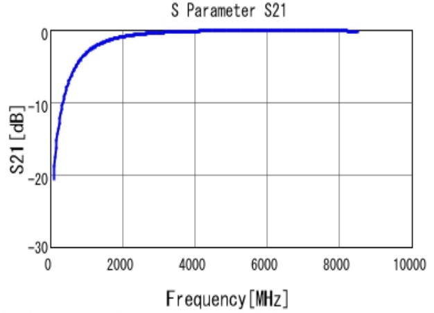
■ GRM1555C1H1R5BA01 S21 DCOV, 25degC
