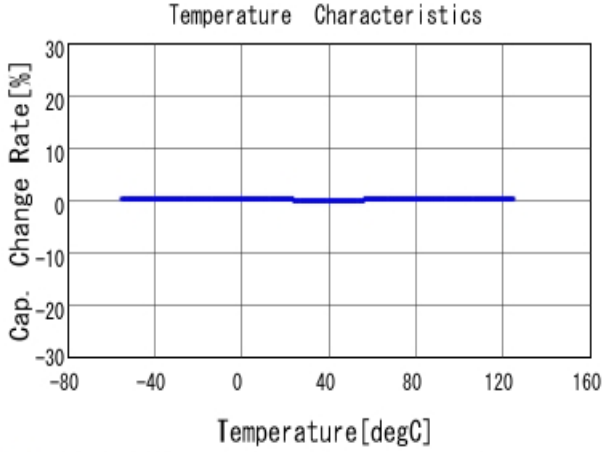
■ GRM1555C1H1R5BA01 C-Temp. capchange, DCOV, AC1Vrms
