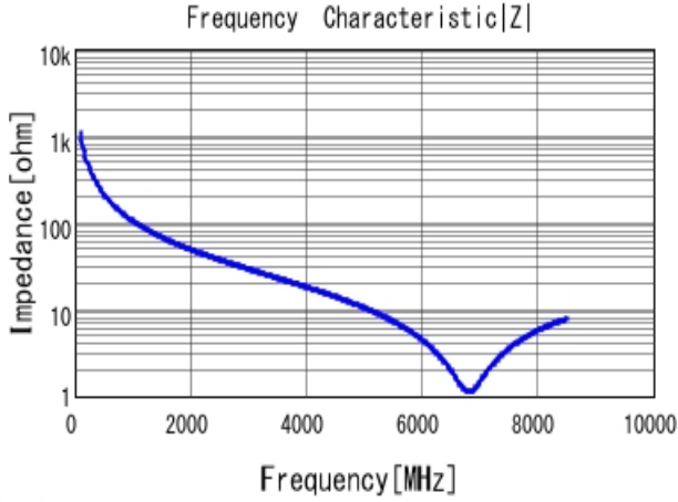
■ GRM1555C1H1R5BA01 |Z| DCOV, 25degC
