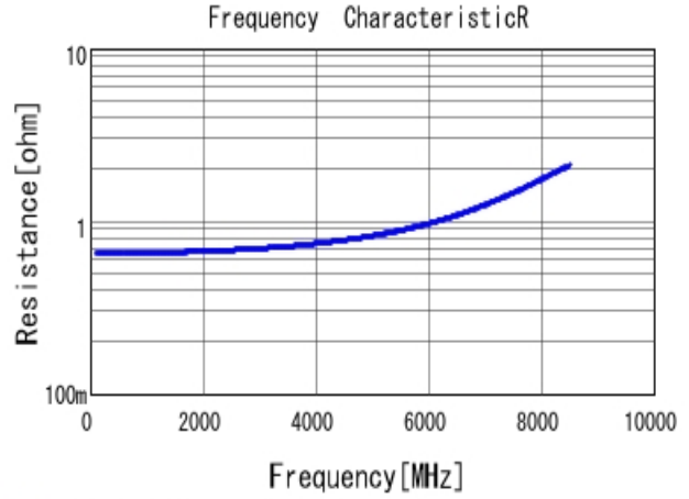
■ GRM1555C1H1R3CA01 R DCOV, 25degC
