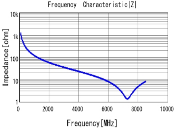
■ GRM1555C1H1R3CA01 |Z| DCOV, 25degC
