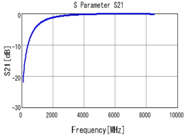
■ GRM1555C1H1R3CA01 S21 DCOV, 25degC
