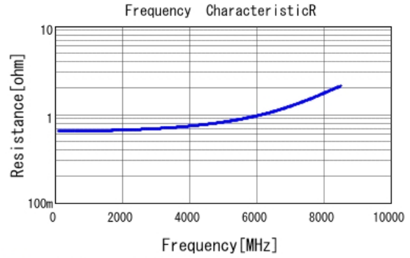
■ GRM1555C1H1R2CA01 R DCOV, 25degC
