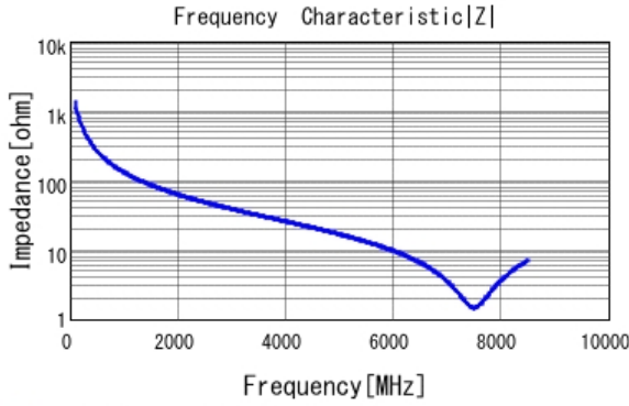
■ GRM1555C1H1R2CA01 |Z| DCOV, 25degC
