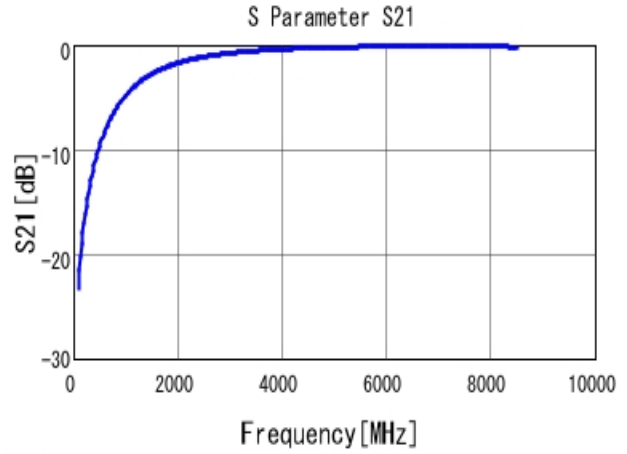
■ GRM1555C1H1R1WA01 S21 DCOV, 25degC
