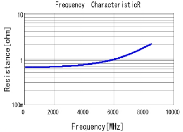
■ GRM1555C1H1R1WA01 R DCOV, 25degC
