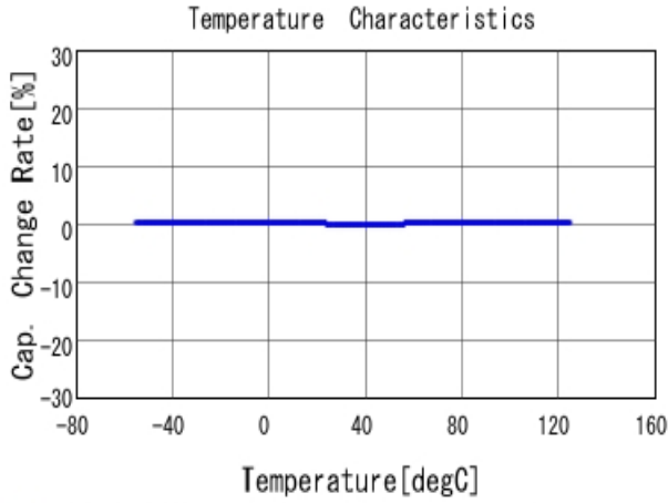
■ GRM1555C1H1R1WA01 C-Temp. capchange, DCOV, AC1Vrms
