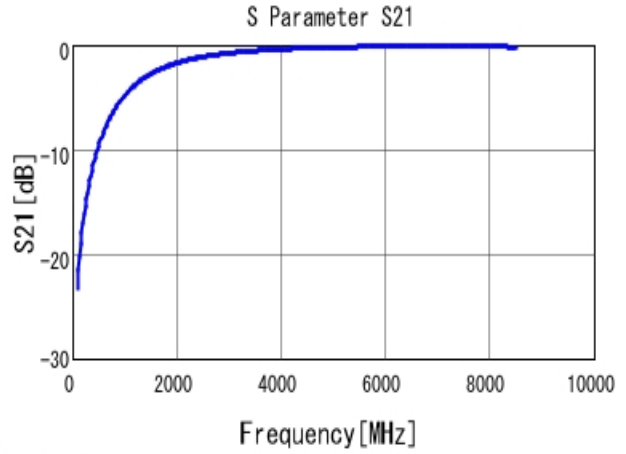
■ GRM1555C1H1R1BA01 S21 DCOV, 25degC
