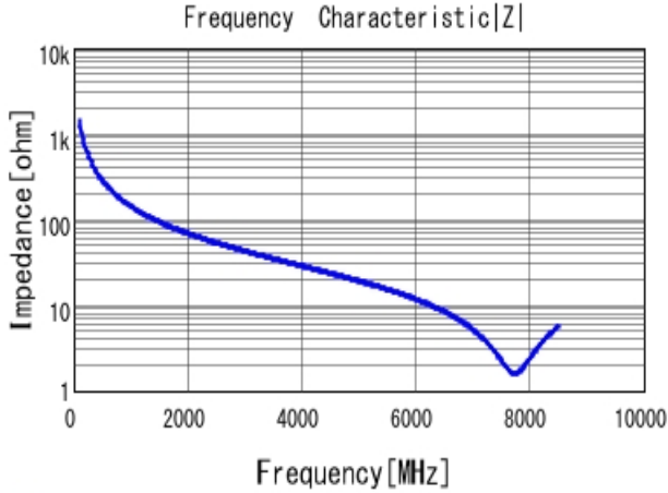
■ GRM1555C1H1R1BA01 |Z| DCOV, 25degC
