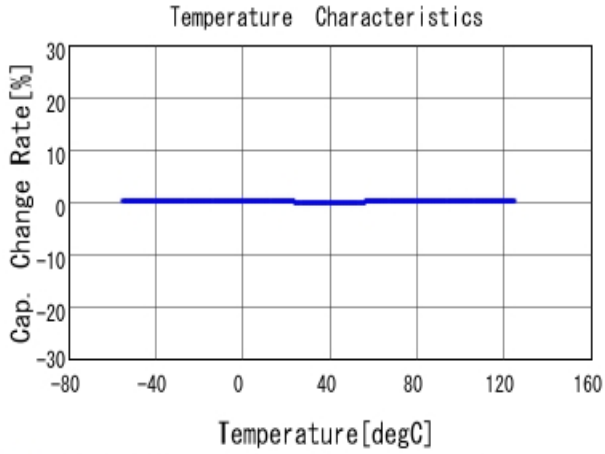
■ GRM1555C1H1R1BA01 C-Temp. capchange, DCOV, AC1Vrms
