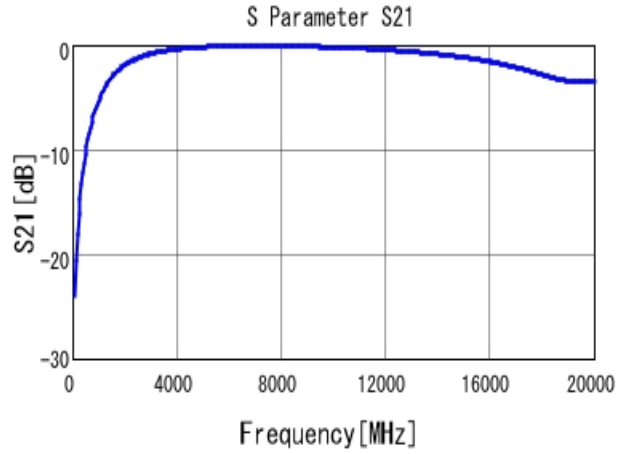
■ GRM1555C1H1R0CA01 S21 DCOV, 25degC
