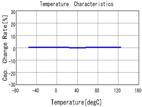
■ GRM1555C1H1R0CA01 C-Temp. capchange, DCOV, AC1Vrms
