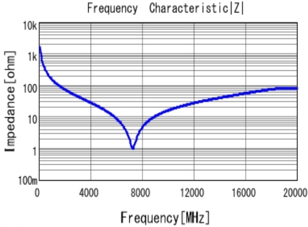
■ GRM1555C1H1R0CA01 |Z| DCOV, 25degC
