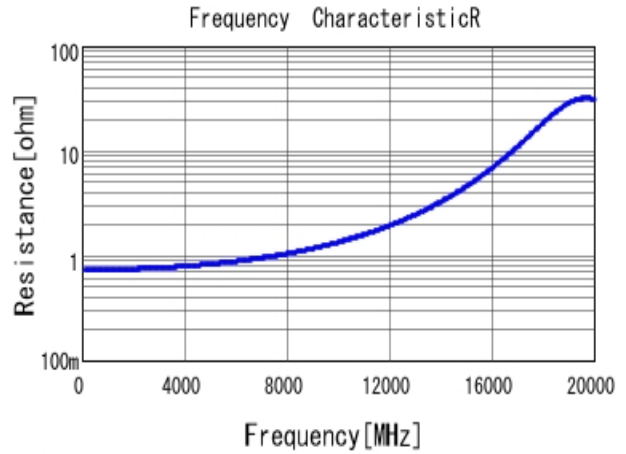
■ GRM1555C1H1R0BA01 R DCOV, 25degC
