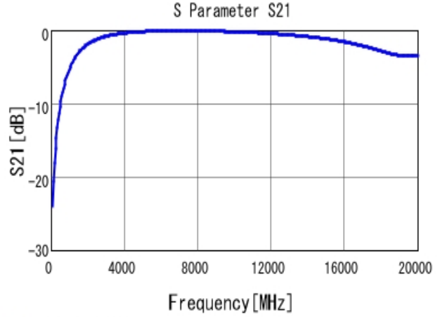
■ GRM1555C1H1R0BA01 S21 DCOV, 25degC
