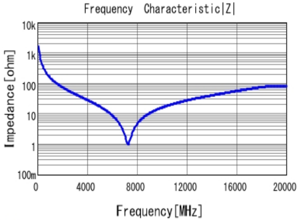
■ GRM1555C1H1R0BA01 |Z| DCOV, 25degC
