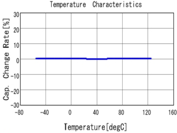
■ GRM1555C1H1R0BA01 C-Temp. capchange, DCOV, AC1Vrms
