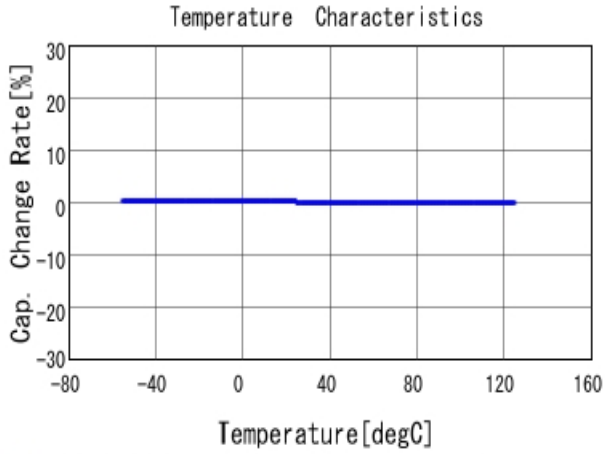
■ GRM1555C1H181JA01 C-Temp. capchange, DCOV, AC1Vrms
