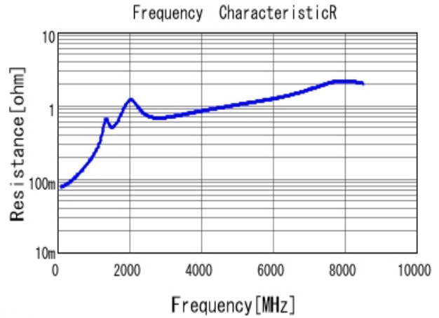
■ GRM1555C1H181JA01 R DCOV, 25degC
