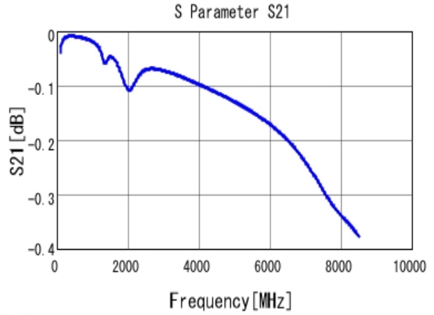
■ GRM1555C1H181JA01 S21 DCOV, 25degC
