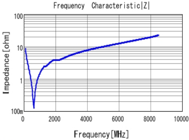
■ GRM1555C1H181GA01 |Z| DCOV, 25degC
