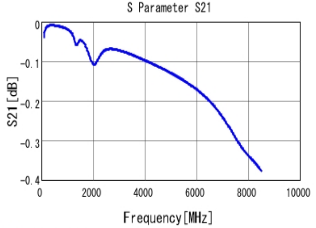
■ GRM1555C1H181GA01 S21 DCOV, 25degC
