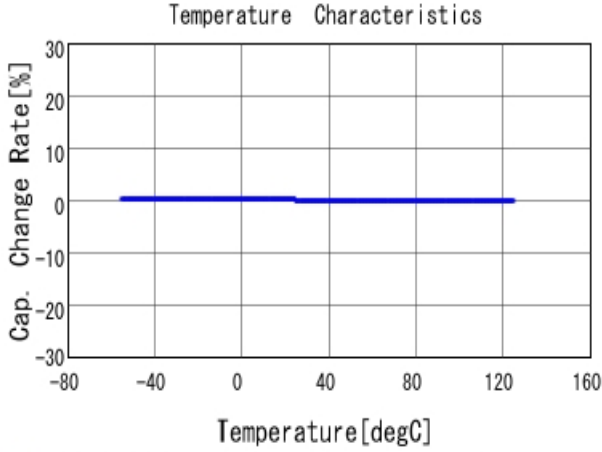
■ GRM1555C1H181GA01 C-Temp. capchange, DCOV, AC1Vrms
