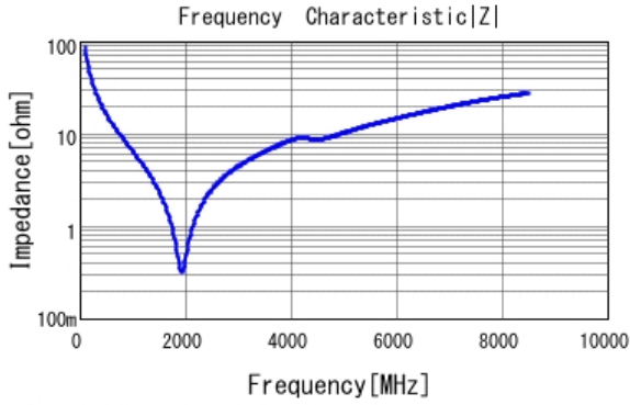
■ GRM1555C1H180JA01 |Z| DCOV, 25degC
