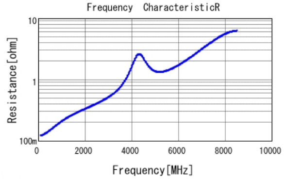
■ GRM1555C1H180JA01 R DCOV, 25degC
