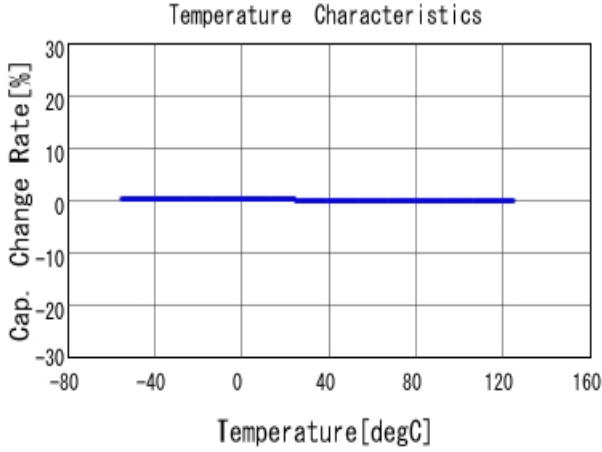
■ GRM1555C1H180GA01 C-Temp. capchange, DCOV, AC1Vrms
