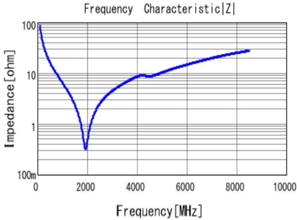
■ GRM1555C1H180GA01 |Z| DC0V, 25degC
