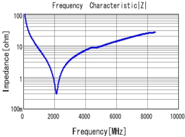
■ GRM1555C1H160JA01 |Z| DCOV, 25degC
