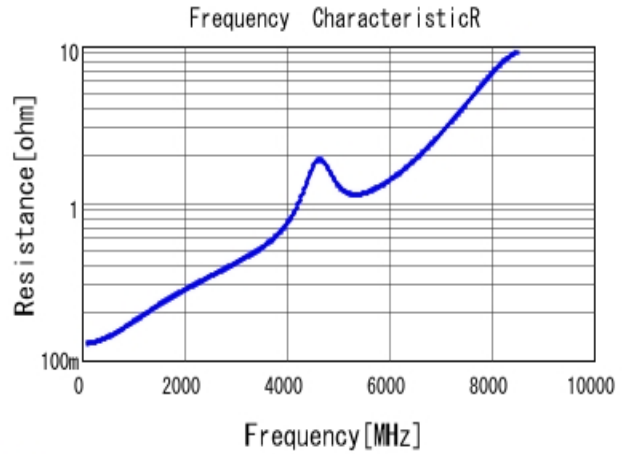
■ GRM1555C1H160JA01 R DCOV, 25degC
