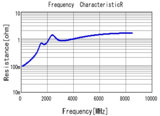
■ GRM1555C1H151JA01 R DCOV, 25degC
