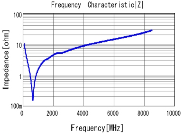
■ GRM1555C1H151GA01 |Z| DCOV, 25degC
