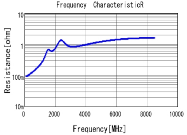
■ GRM1555C1H151GA01 R DCOV, 25degC
