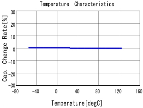
■ GRM1555C1H150JA01 C-Temp. capchange, DCOV, AC1Vrms
