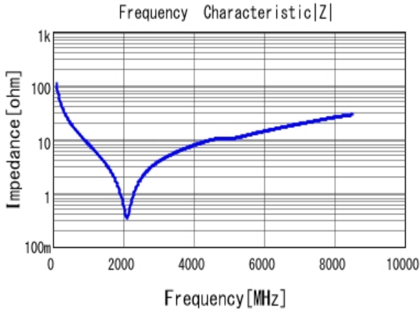
■ GRM1555C1H150JA01 |Z| DCOV, 25degC
