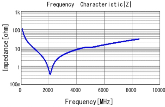
■ GRM1555C1H150GA01 |Z| DCOV, 25degC
