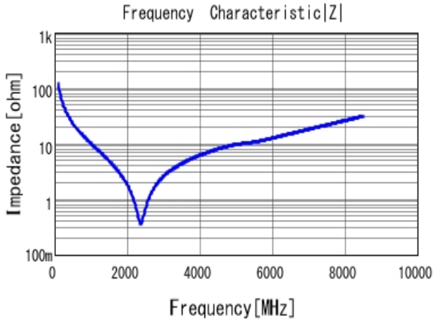
■ GRM1555C1H130JA01 |Z| DCOV, 25degC
