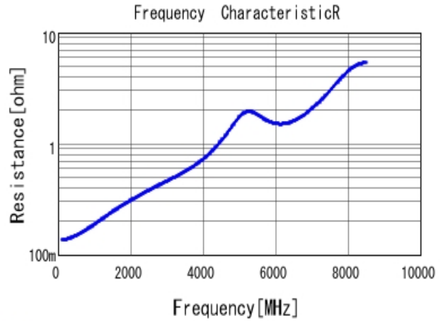
■ GRM1555C1H130JA01 R DCOV, 25degC
