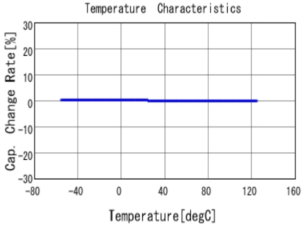
■ GRM1555C1H130JA01 C-Temp. capchange, DCOV, AC1Vrms
