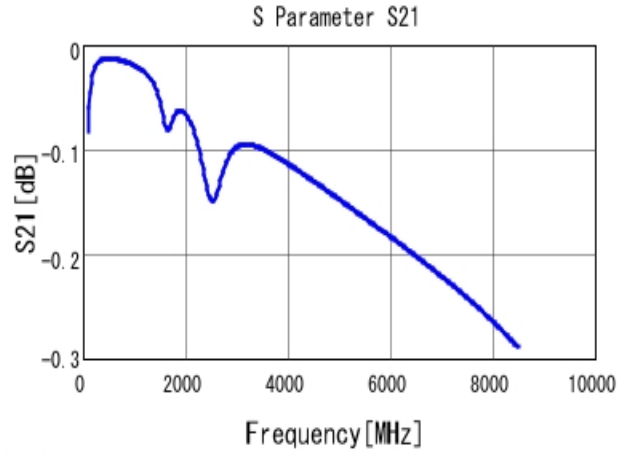
■ GRM1555C1H121JA01 S21 DCOV, 25degC
