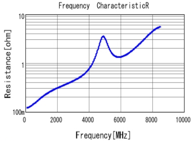
■ GRM1555C1H120JA01 R DCOV, 25degC
