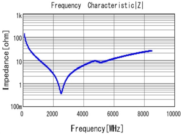
■ GRM1555C1H120JA01 |Z| DCOV, 25degC
