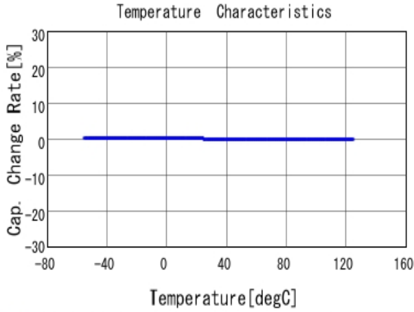
■ GRM1555C1H120JA01 C-Temp. capchange, DCOV, AC1Vrms
