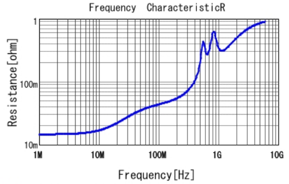
■ GRM1555C1H102JA01 R DCOV, 25degC
