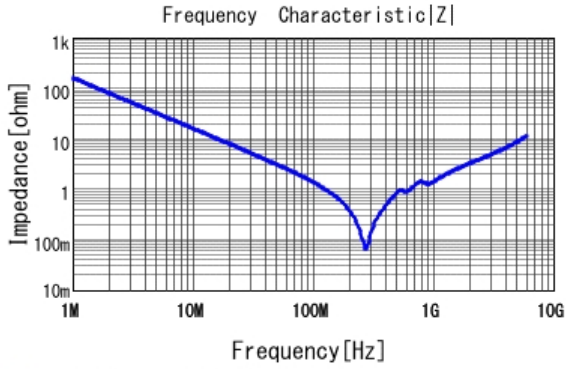
■ GRM1555C1H102JA01 |Z| DCOV, 25degC
