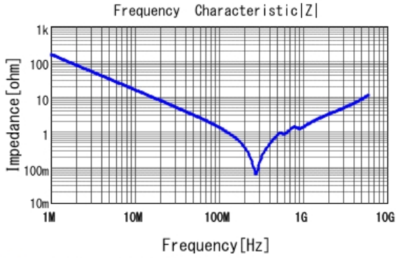
■ GRM1555C1H102GA01 |Z| DCOV, 25degC
