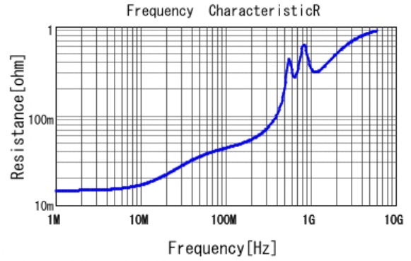
■ GRM1555C1H102GA01 R DCOV, 25degC
