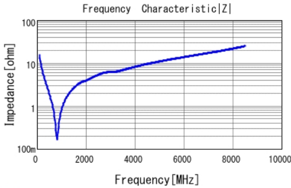
■ GRM1555C1H101JA01 |Z| DCOV, 25degC
