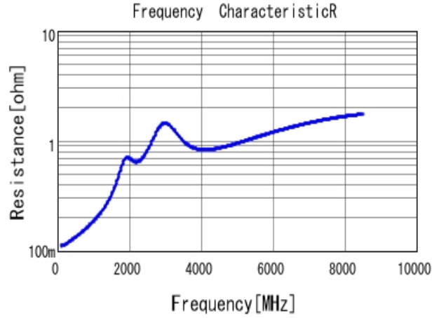
■ GRM1555C1H101GA01 R DCOV, 25degC
