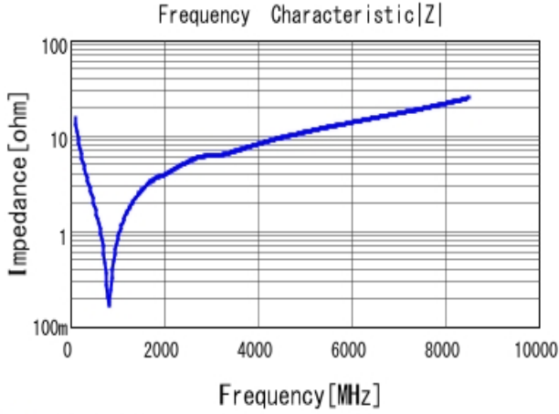
■ GRM1555C1H101GA01 |Z| DCOV, 25degC
