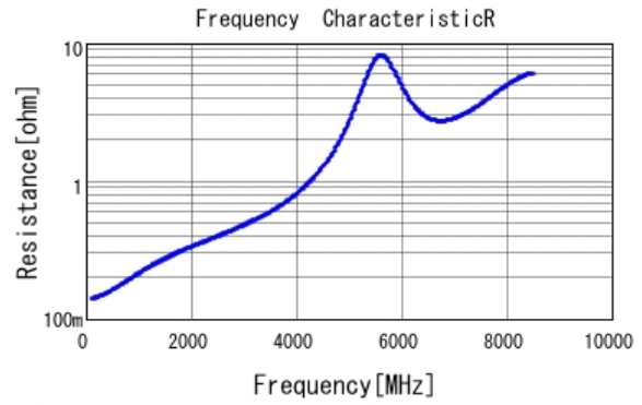
■ GRM1555C1H100JA01 R DCOV, 25degC
