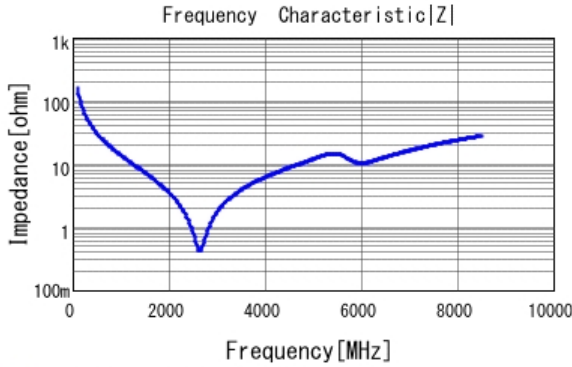
■ GRM1555C1H100GA01 |Z| DCOV, 25degC
