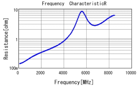
■ GRM1555C1H100GA01 R DCOV, 25degC
