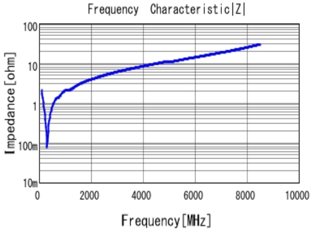
■ GRM1555C1E681JA01 |Z| DCOV, 25degC
