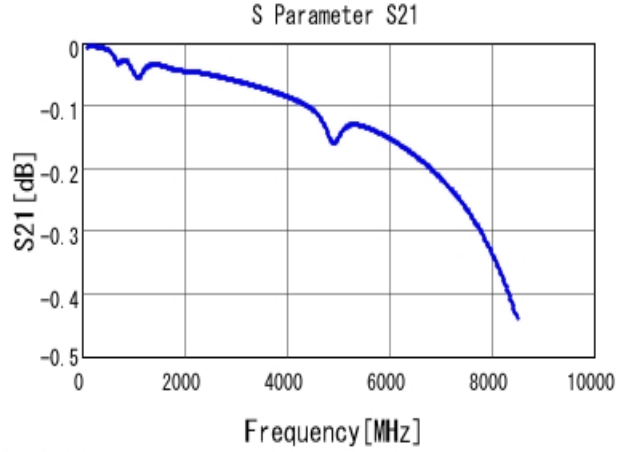
■ GRM1555C1E681JA01 S21 DCOV, 25degC
