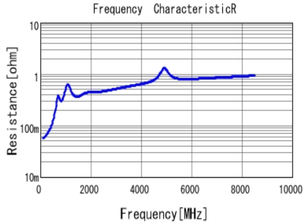
■ GRM1555C1E681JA01 R DCOV, 25degC
