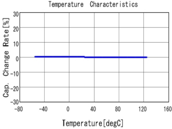
■ GRM1555C1E681JA01 C-Temp. capchange, DCOV, AC1Vrms
