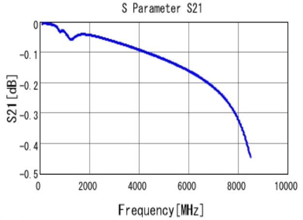
■ GRM1555C1E561JA01 S21 DCOV, 25degC
