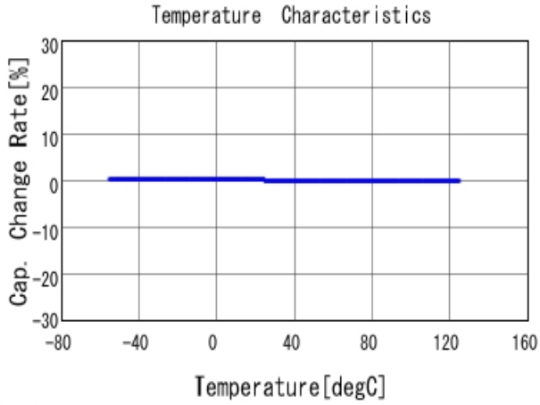
■ GRM1555C1E561JA01 C-Temp. capchange, DCOV, AC1Vrms
