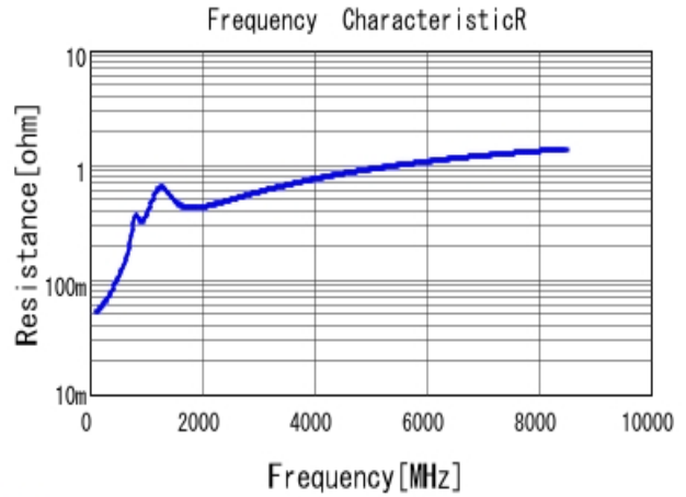
■ GRM1555C1E561JA01 R DCOV, 25degC
