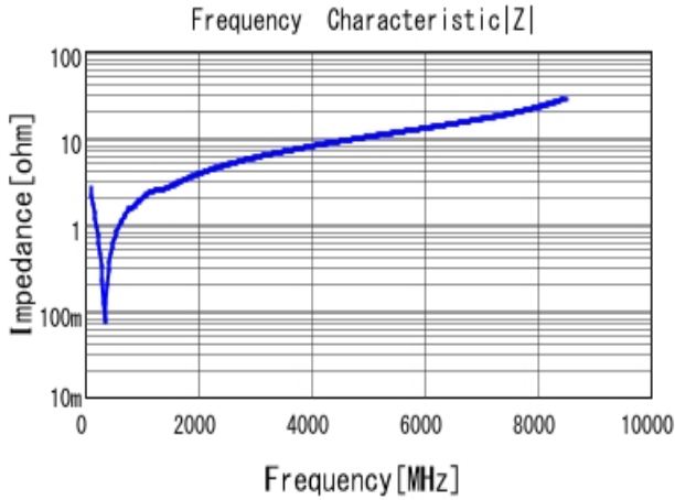
■ GRM1555C1E561JA01 |Z| DCOV, 25degC
