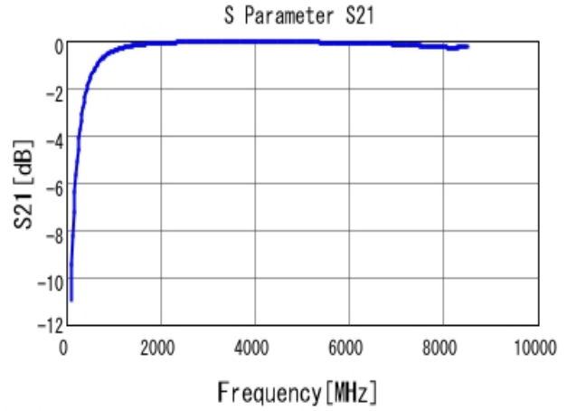
■ GRM1555C1E4R7CA01 S21 DCOV, 25degC
