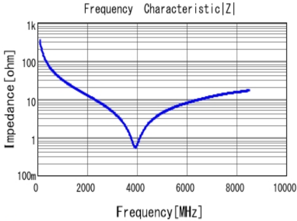
■ GRM1555C1E4R7CA01 |Z| DC0V, 25degC
