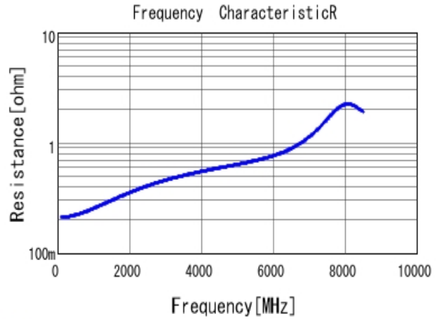
■ GRM1555C1E4R7CA01 R DC0V, 25degC
