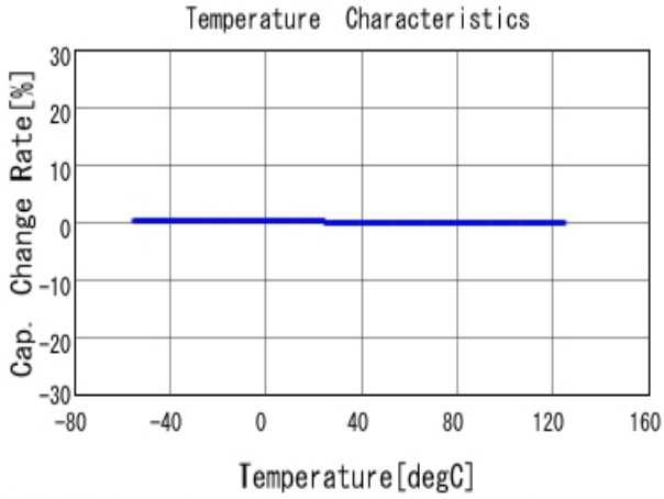
■ GRM1555C1E471JA01 C-Temp. capchange, DCOV, AC1Vrms
