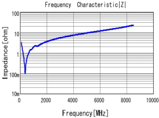
■ GRM1555C1E471JA01 |Z| DCOV, 25degC
