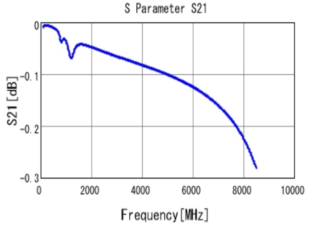
■ GRM1555C1E471JA01 S21 DCOV, 25degC
