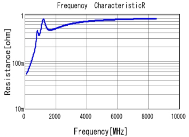
■ GRM1555C1E471JA01 R DCOV, 25degC
