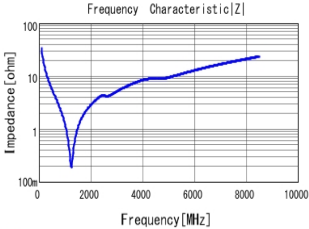
■ GRM1555C1E470JA01 |Z| DC0V, 25degC
