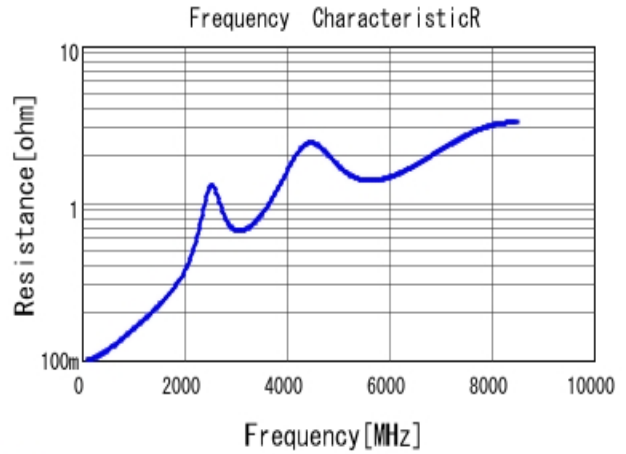
■ GRM1555C1E470JA01 R DC0V, 25degC
