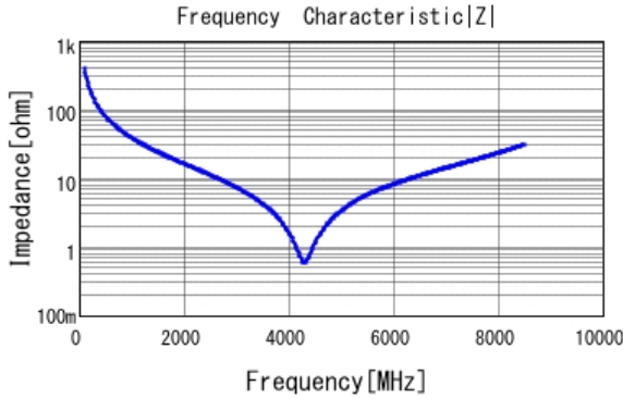
■ GRM1555C1E3R9CA01 |Z| DCOV, 25degC
