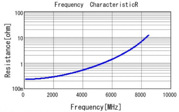
■ GRM1555C1E3R9CA01 R DCOV, 25degC
