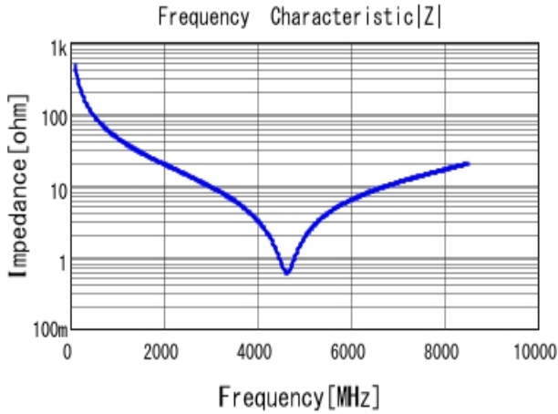
■ GRM1555C1E3R3CA01 |Z| DC0V, 25degC
