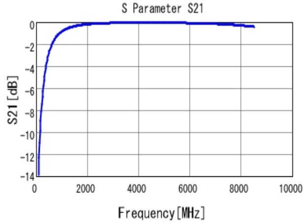
■ GRM1555C1E3R3CA01 S21 DCOV, 25degC
