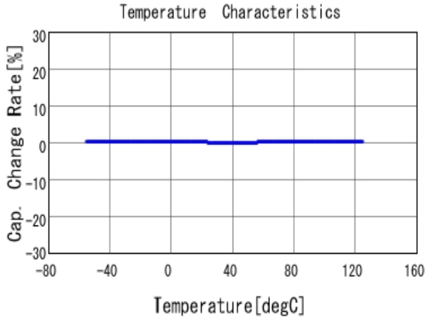
■ GRM1555C1E3R3CA01 C-Temp. capchange, DCOV, AC1Vrms
