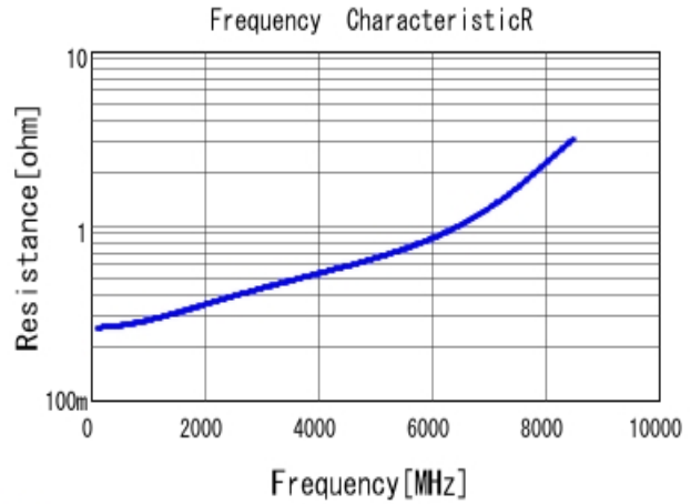
■ GRM1555C1E3R3CA01 R DC0V, 25degC
