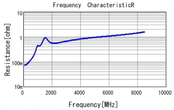
■ GRM1555C1E331JA01 R DCOV, 25degC
