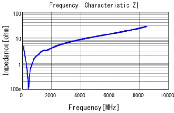
■ GRM1555C1E331JA01 |Z| DCOV, 25degC
