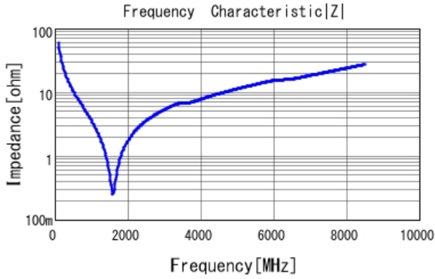
GRM1555C1E270JA01 |Z| DCOV, 25degC
