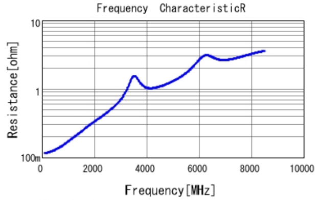
GRM1555C1E270JA01 R DCOV, 25degC
