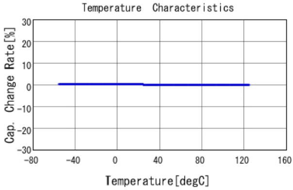
GRM1555C1E270JA01 C-Temp. capchange, DCOV, AC1Vrms
