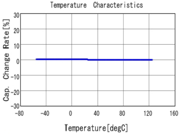
■ GRM1555C1E221JA01 C-Temp. capchange, DCOV, AC1Vrms
