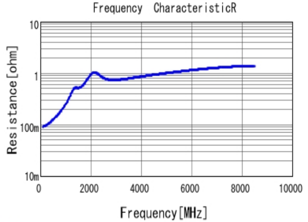
■ GRM1555C1E221JA01 R DCOV, 25degC
