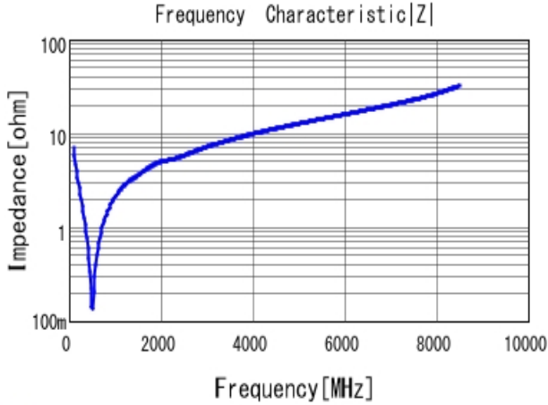
■ GRM1555C1E221JA01 |Z| DCOV, 25degC
