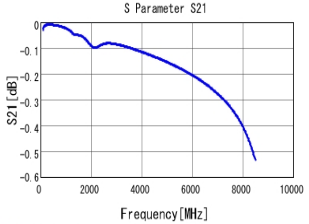
■ GRM1555C1E221JA01 S21 DCOV, 25degC
