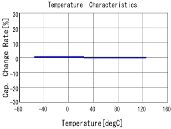
■ GRM1555C1E220JA01 C-Temp. capchange, DCOV, AC1Vrms
