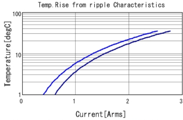
GRM153R61A105ME95 Temp. rise ■ 500kHz ■ 1MHz
