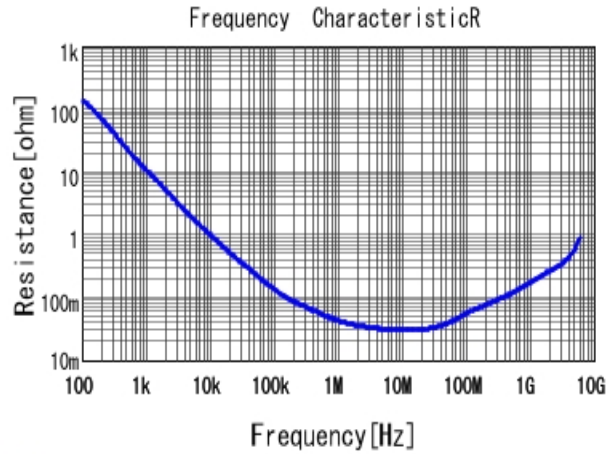
■ GRM152R61A104KE19 R DCOV, 25degC
