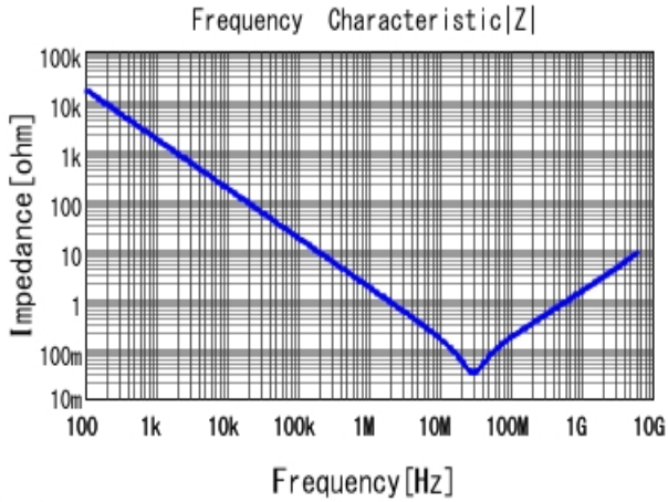
■ GRM152R61A104KE19 |Z| DCOV, 25degC
