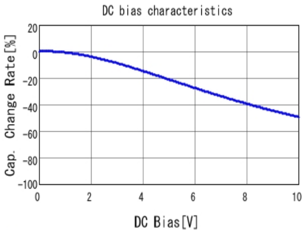
■ GRM152R61A104KE19 C-DC bias capchange, 25.0degC, AC1V
