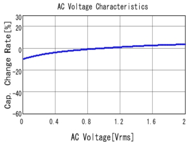
■ GRM152R61A104KE19 C-AC Voltage capchange, DCOV, 25.0d
