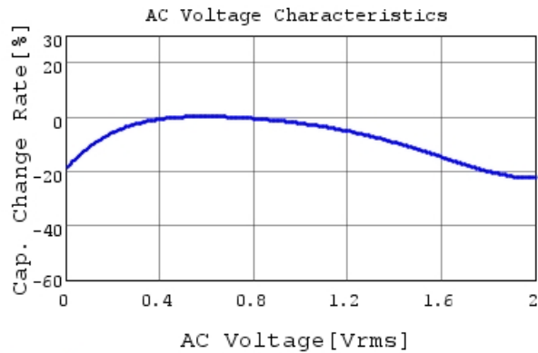
GRM035R60J475ME15 C-AC Voltage capchange, Dc
