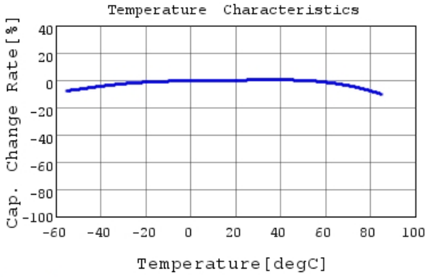
GRM035R60J475ME15 C-Temp. capchange, DC0.0V,
