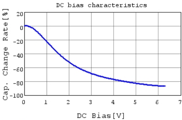
GRM035R60J475ME15 C-DC bias capchange, 25.0c
