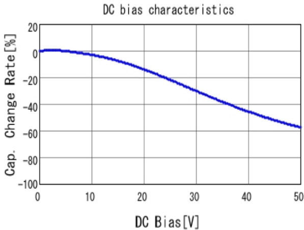
■ GRM033R71H331MA12 C-DC bias capchange, 25.0degC, AC1.
