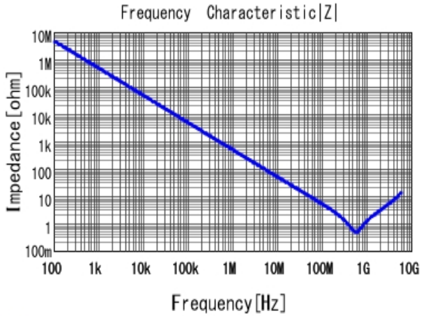
■ GRM033R71H331MA12 |Z| DCOV, 25degC
