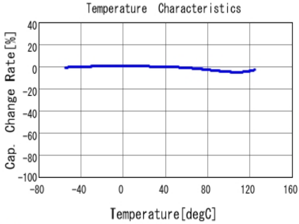
■ GRM033R71H331MA12 C-Temp. capchange, DCO. 0V, AC1.0Vrm
