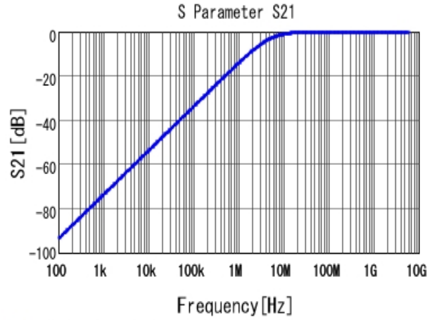
■ GRM033R71H331MA12 S21 DCOV, 25degC
