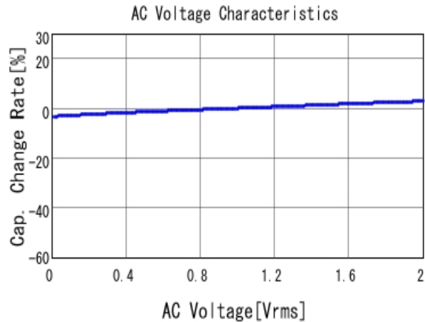
■ GRM033R71H331MA12 C-AC Voltage capchange, DCOV, 25.0d
