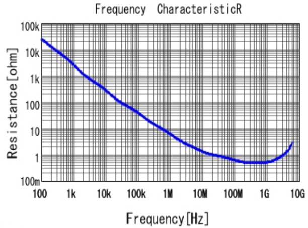
■ GRM033R71H331MA12 R DCOV, 25degC
