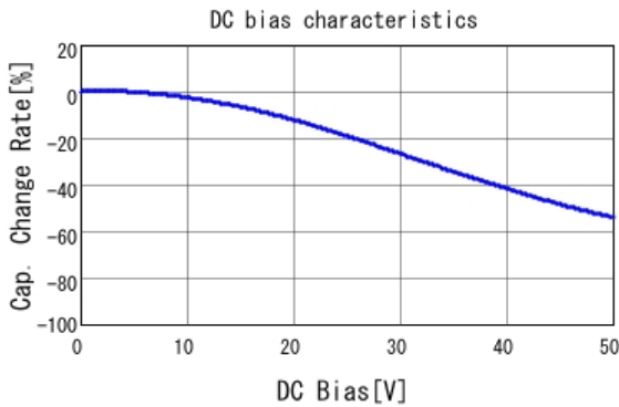
■ GRM033R71H221KA12 C-DC bias capchange, 25.0degC, AC1.
