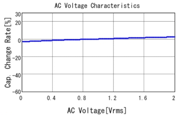
■ GRM033R71H221KA12 C-AC Voltage capchange, DCOV, 25.0d
