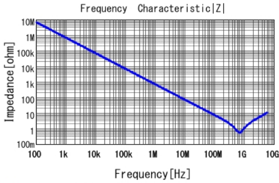
■ GRM033R71H221KA12 |Z| DCOV, 25degC
