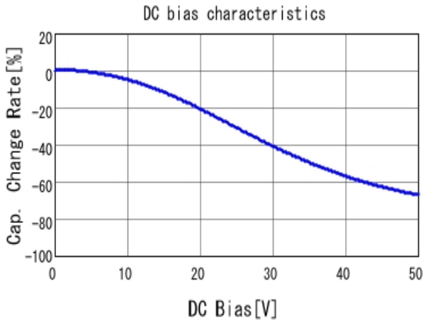
■ GRM033R71H102MA12 C-DC bias capchange, 25.0degC, AC1.
