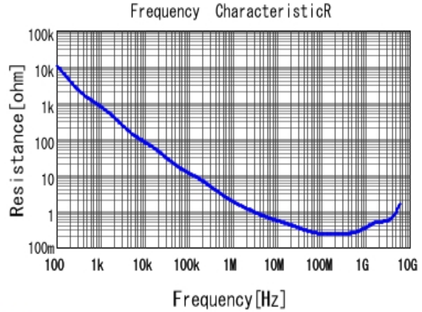
■ GRM033R71H102MA12 R DCOV, 25degC
