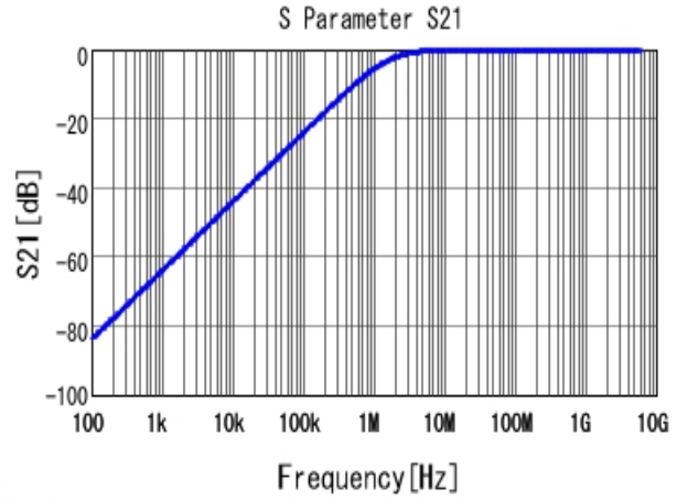
■ GRM033R71H102MA12 S21 DCOV, 25degC
