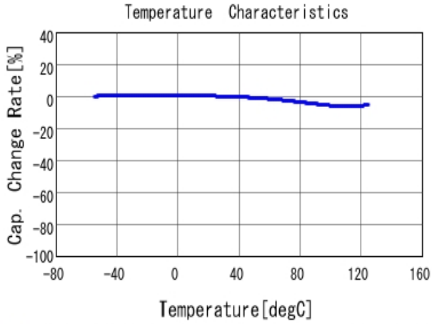
■ GRM033R71H102MA12 C-Temp. capchange, DCO. 0V, AC1.0Vrm
