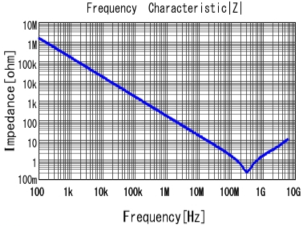
■ GRM033R71H102MA12 |Z| DCOV, 25degC
