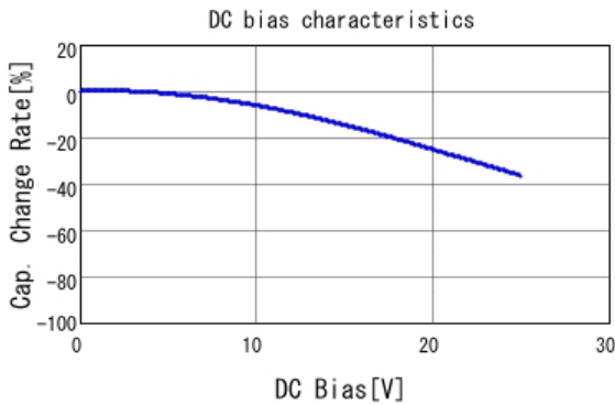
■ GRM033R71E152KA01 C-DC bias capchange, 25.0degC, AC1.
