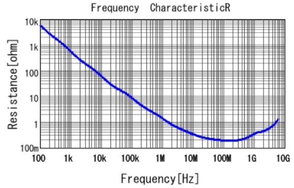
■ GRM033R71E152KA01 R DCOV, 25degC
