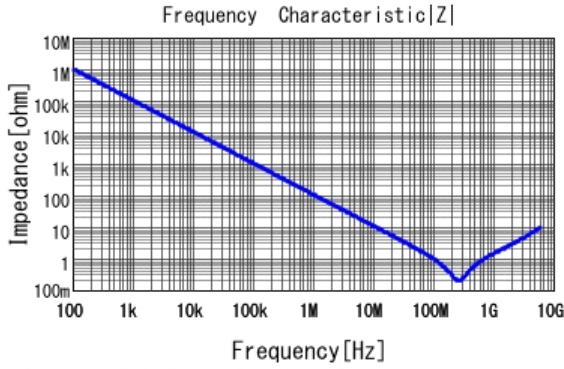
■ GRM033R71E152KA01 |Z| DCOV, 25degC
