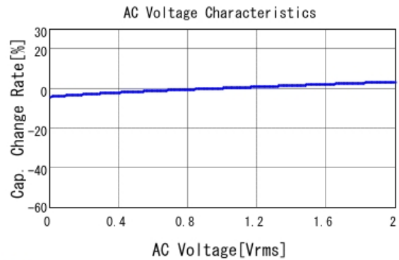
■ GRM033R71E152KA01 C-AC Voltage capchange, DCOV, 25.0d
