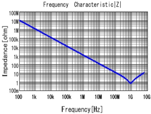
■ GRM033R71E151KA01 |Z| DCOV, 25degC
