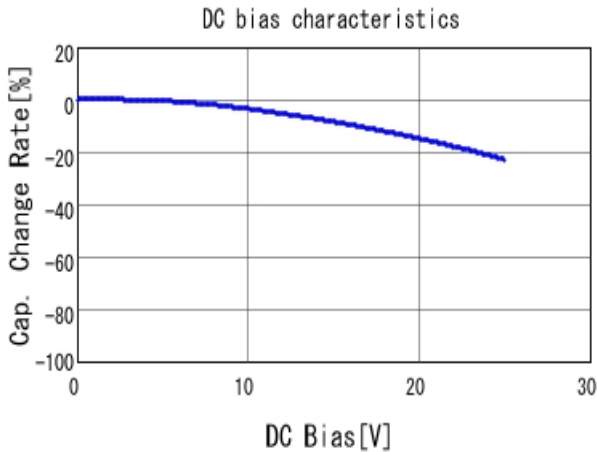
■ GRM033R71E151KA01 C-DC bias capchange, 25.0degC, AC1.
