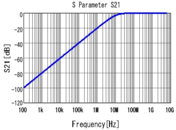
■ GRM033R71E151KA01 S21 DCOV, 25degC
