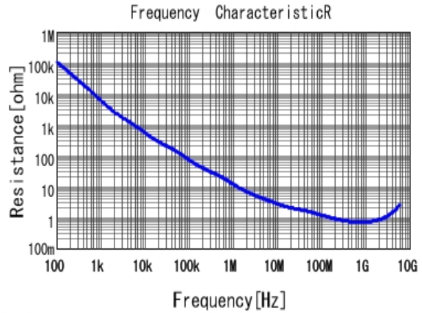
■ GRM033R71E151KA01 R DCOV, 25degC
