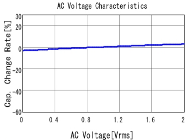
■ GRM033R71E151KA01 C-AC Voltage capchange, DCOV, 25.0d
