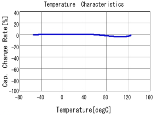
■ GRM033R71E151KA01 C-Temp. capchange, DCO. 0V, AC1.0V rm
