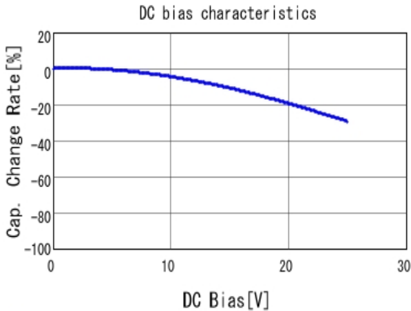
■ GRM033R71E102KA01 C-DC bias capchange, 25.0degC, AC1.
