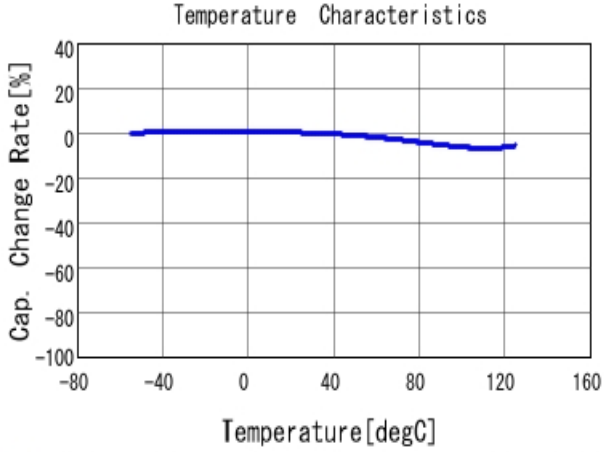
■ GRM033R71E102KA01 C-Temp. capchange, DCO. 0V, AC1.0Vrm
