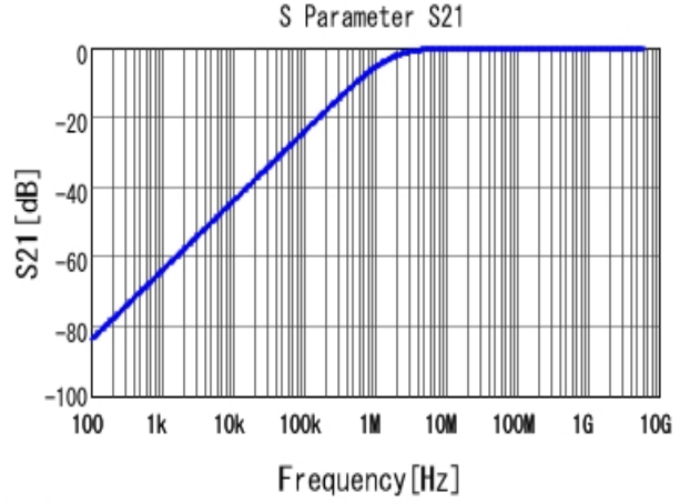
■ GRM033R71E102KA01 S21 DCOV, 25degC
